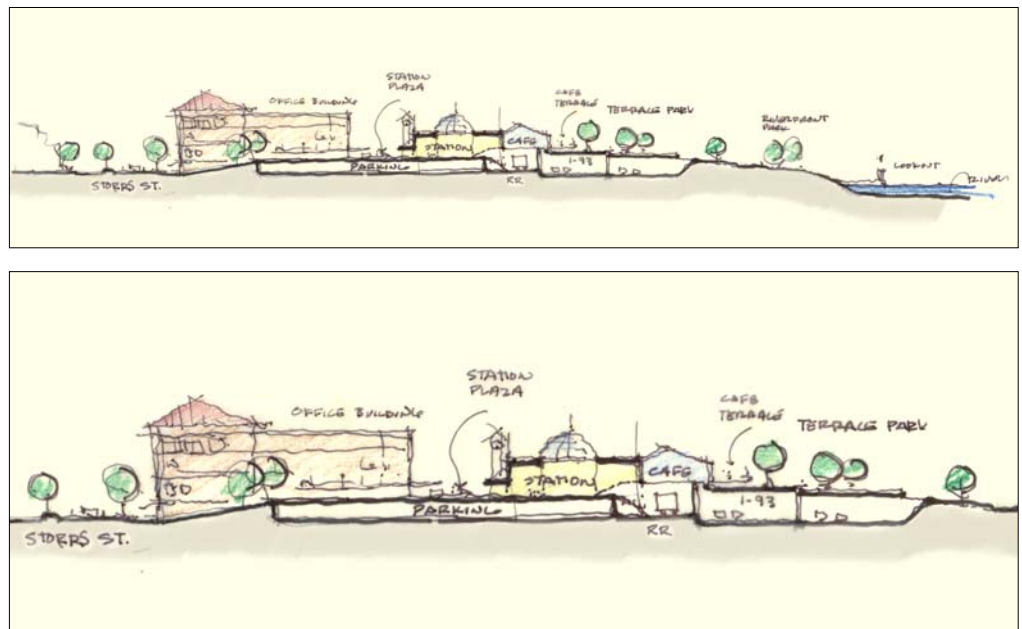
Figure 17. Multimodal Transportation Center – Section View and Detail
